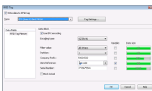
RFID smart label printing in NiceLabel Pro
